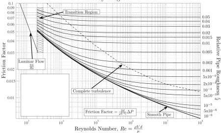
Moody Diagram
